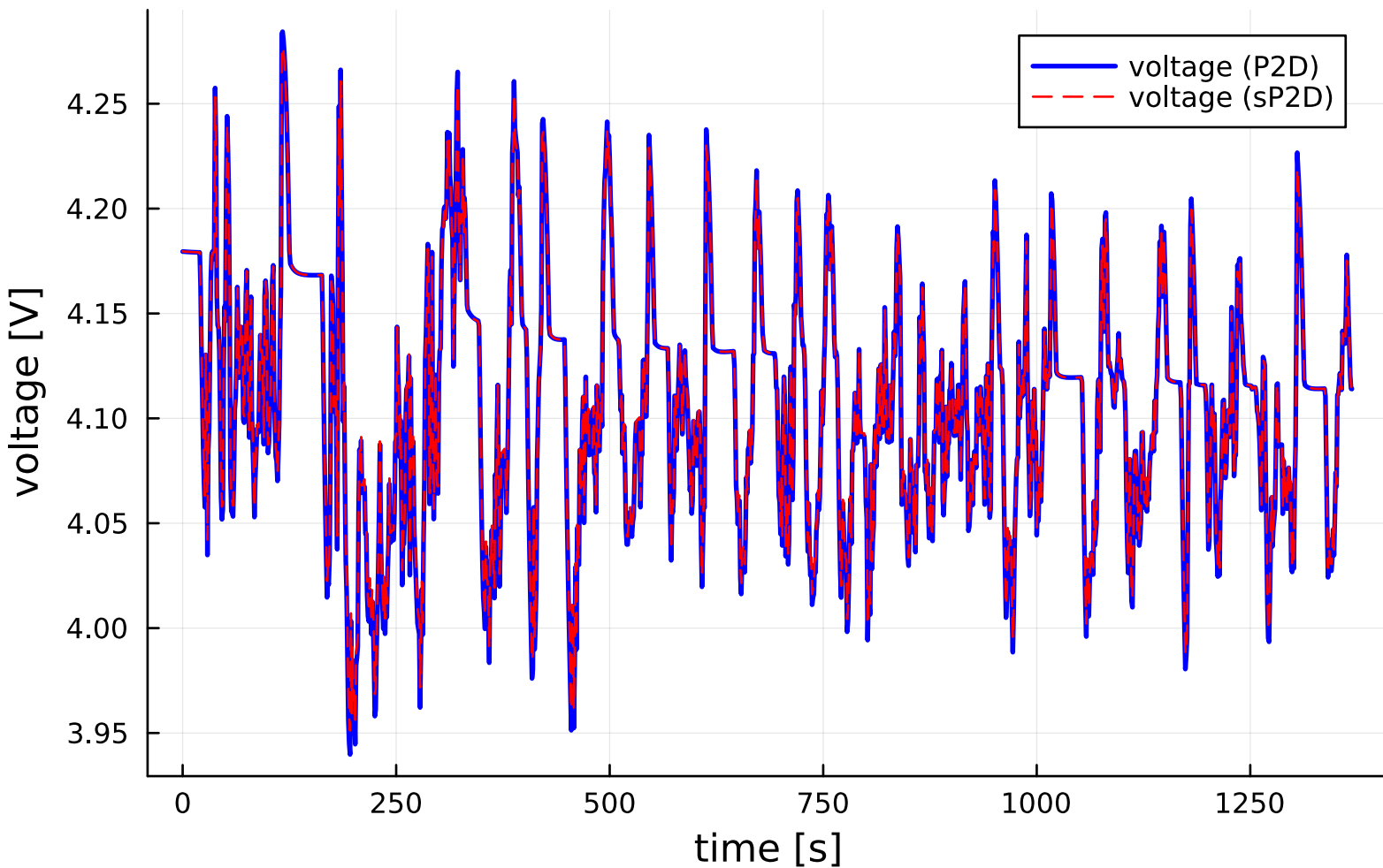
voltage_comparison (P2D vs sP2D)
